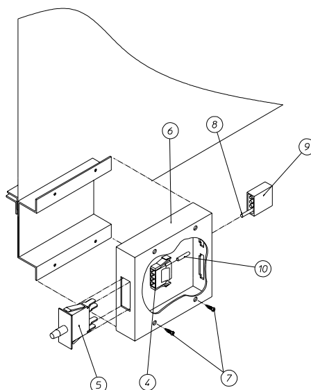
LINT DRAWER SWITCH ASSY
